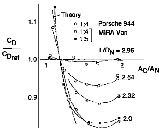
Figure 24 Influence of test-section length L (relative to the hydraulic diameter D_N of the nozzle) and the ratio of collector area ( A_C ) to nozzle area ( A_N ) on measured drag; Porsche 22 m 2 wind tunnel, open test section.
